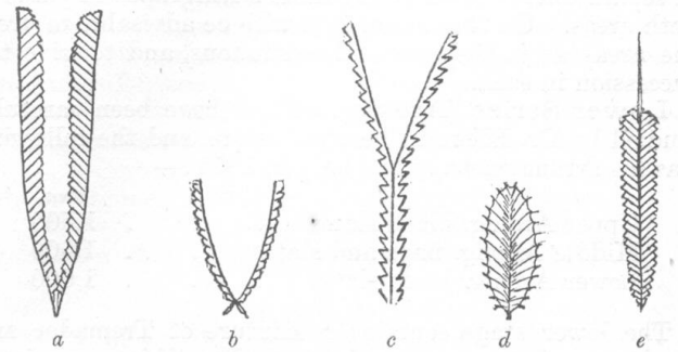
Fig. 9. Ordovician Graptolites.
